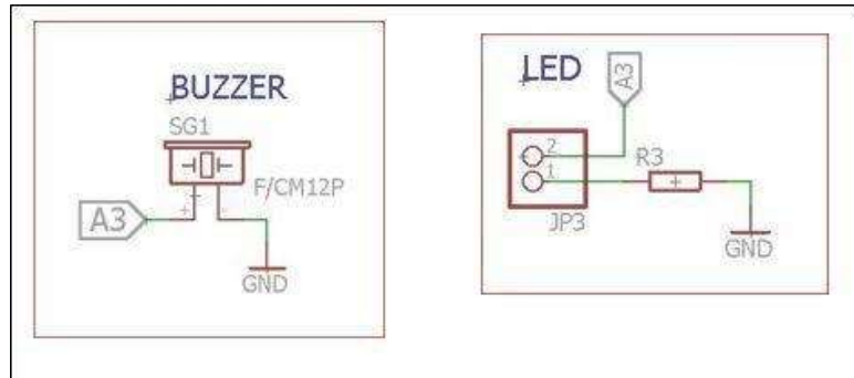
Gambar 5. Rangkain Buzzer dan LED
